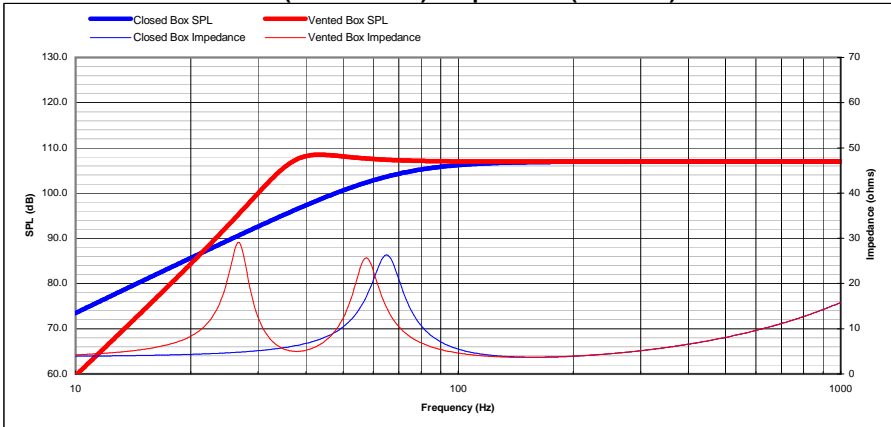
SPL (at 200 Watts) / Impedance (at 1 Watt)
