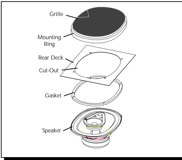
Example of 6" x 9" rear-deck installation
