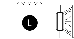
6dB/Octave Low-Pass
