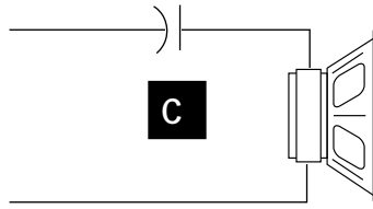
6dB/Octave High-Pass
