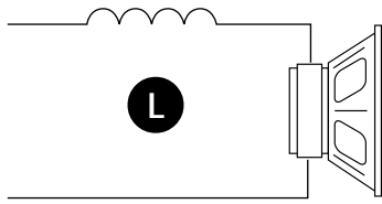
6dB/Octave Low-Pass
