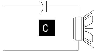
6dB/Octave High-Pass
