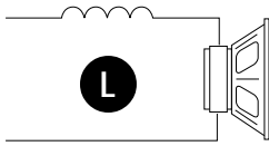
6dB/Octave Low-Pass
